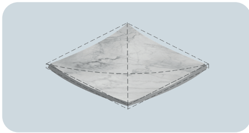
Concavity and Convexity
