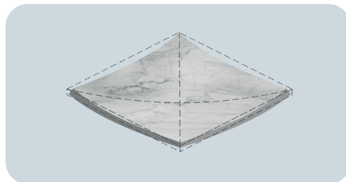
Diagonal Concavity and Convexity
